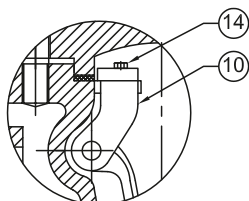
Internally Mounted Hinge
